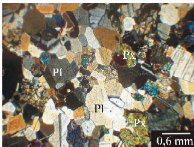
Fig. 13: textura inequigranular seriada (Gabro, Nx)
